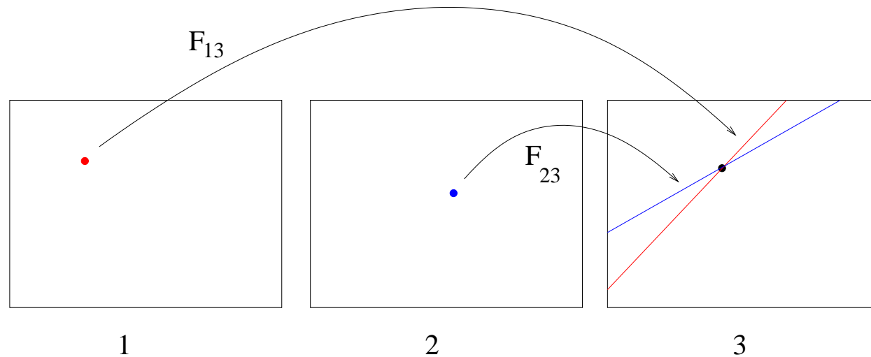
Fig. 17. Point transfer using epipolar constraints between three views.
