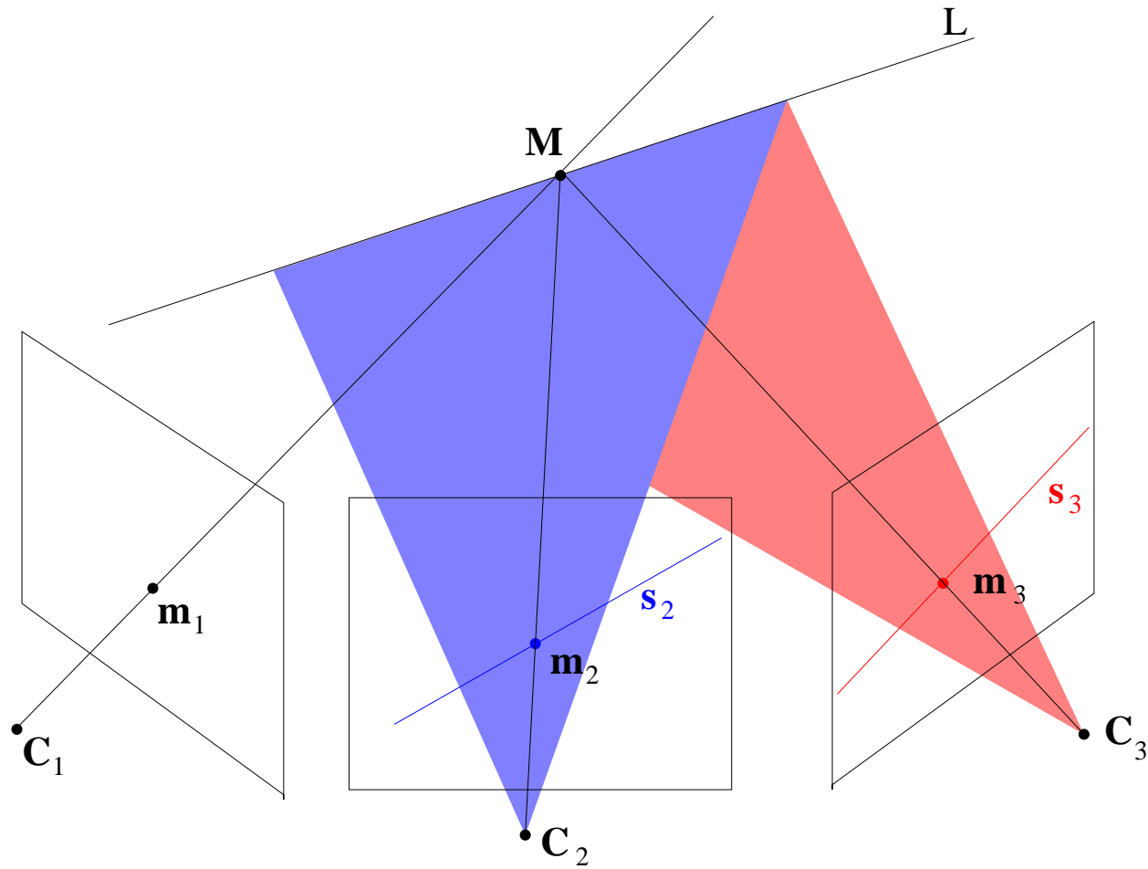
Fig. 18. Two arbitrary lines s_2 and s_3 through corresponding points m_2 and m_3 in the second and third image respectively, define a 3-D line L that must intersect the optical ray of m_1 .
