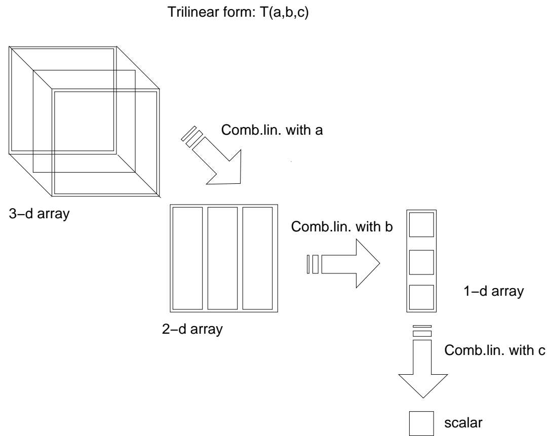
Fig. 19. Action of a trilinear form f(a,b,c) represented by a tensor.
