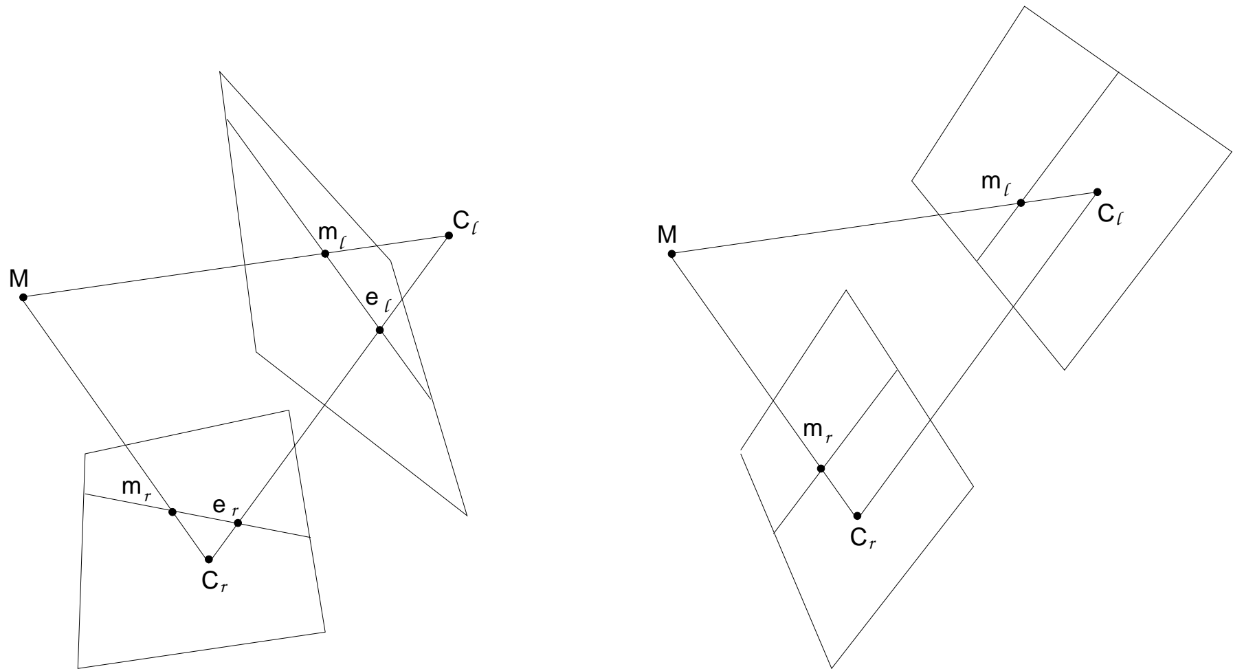
Fig. 13. Epipolar geometry before and after rectification.
