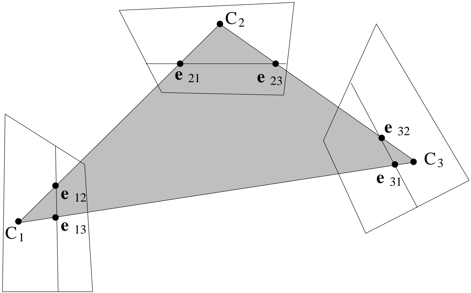
Fig. 16. Trifocal geometry.
