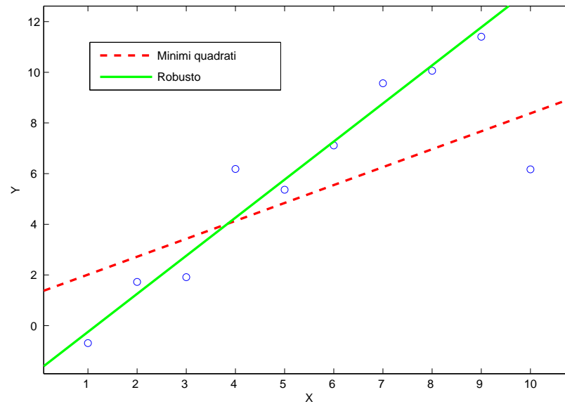
Fig. 17. A single outlier can severely offset the least-squares estimate (red line), whereas the robust estimate (green line) is unaffected.
