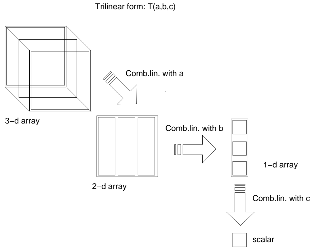
Fig. 16. Action of a trilinear form f(a,b,c) represented by a tensor.
