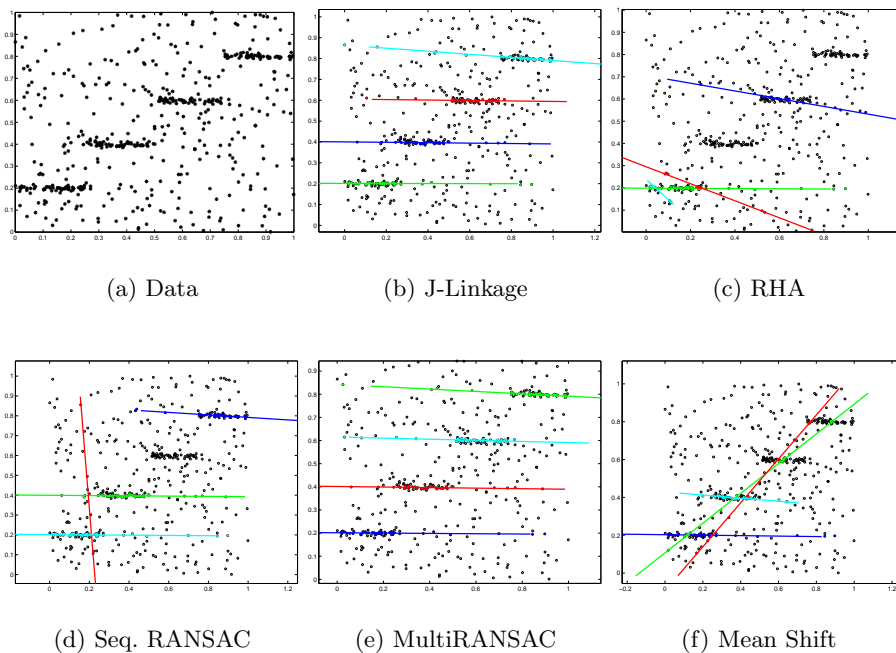
Fig. 7. stair 4 set perturbed with Gaussian noise ( \sigma_n = 0.0075 ) and 60% outliers.
